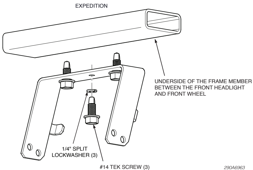
Figure 1 Mounting location on Ford Expedition
