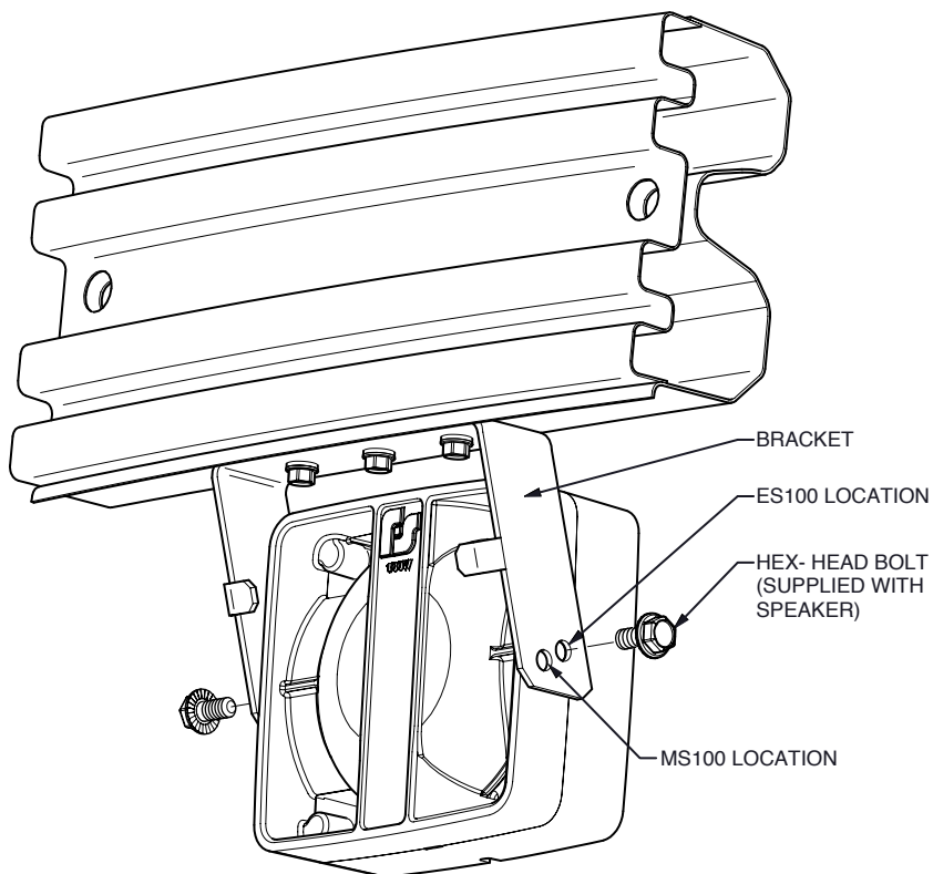
Figure 4 Speaker alignment on Ford Explorer and Police Utility
