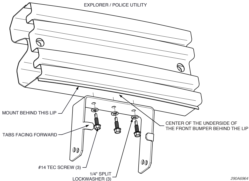
Figure 2 Mounting location on Ford Explorer and Police Utility
