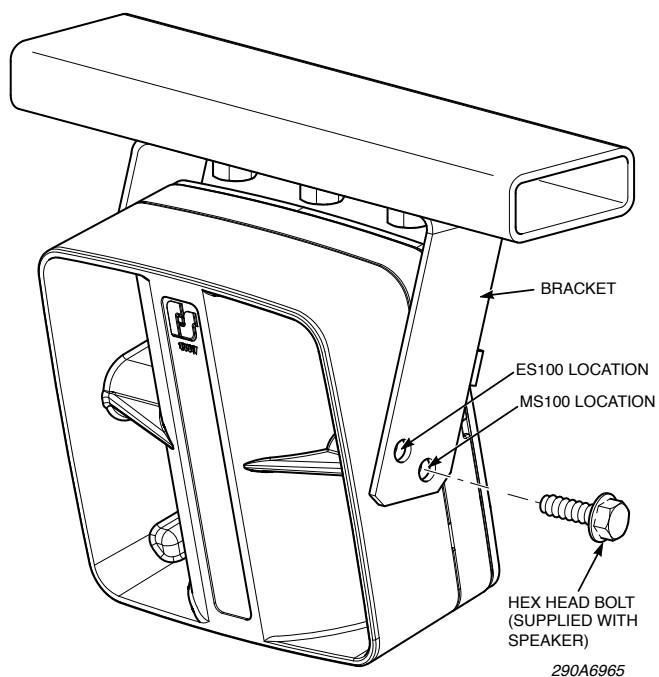
Figure 3 Speaker alignment on Ford Expedition
